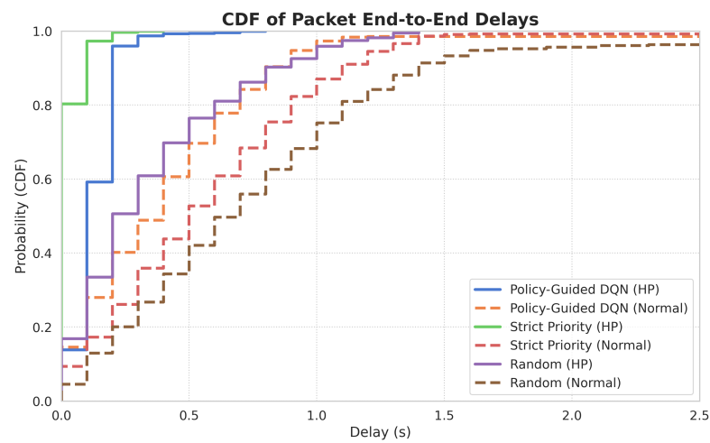
Fig. 3. Cumulative Distribution Function (CDF) of packet end-to-end delays for high-priority and normal-priority traffic classes.
